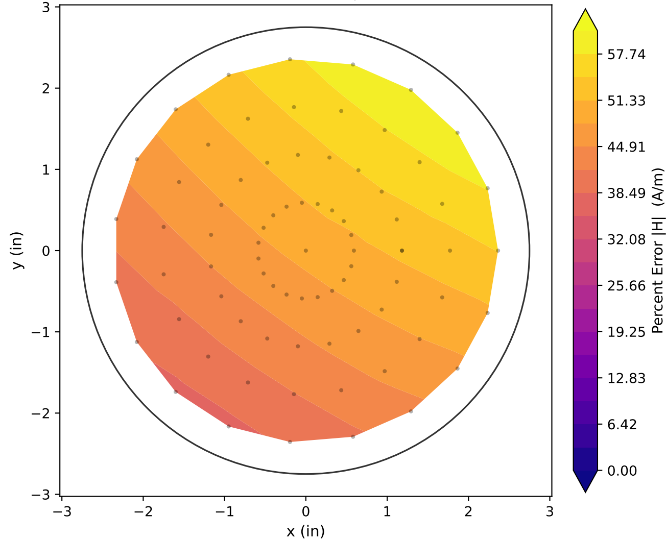
Reconstruction Error Percent — J=66.039 A/in 2 , slice 1
